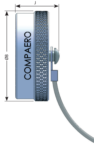
CPA 33 - Receptacle Cover
